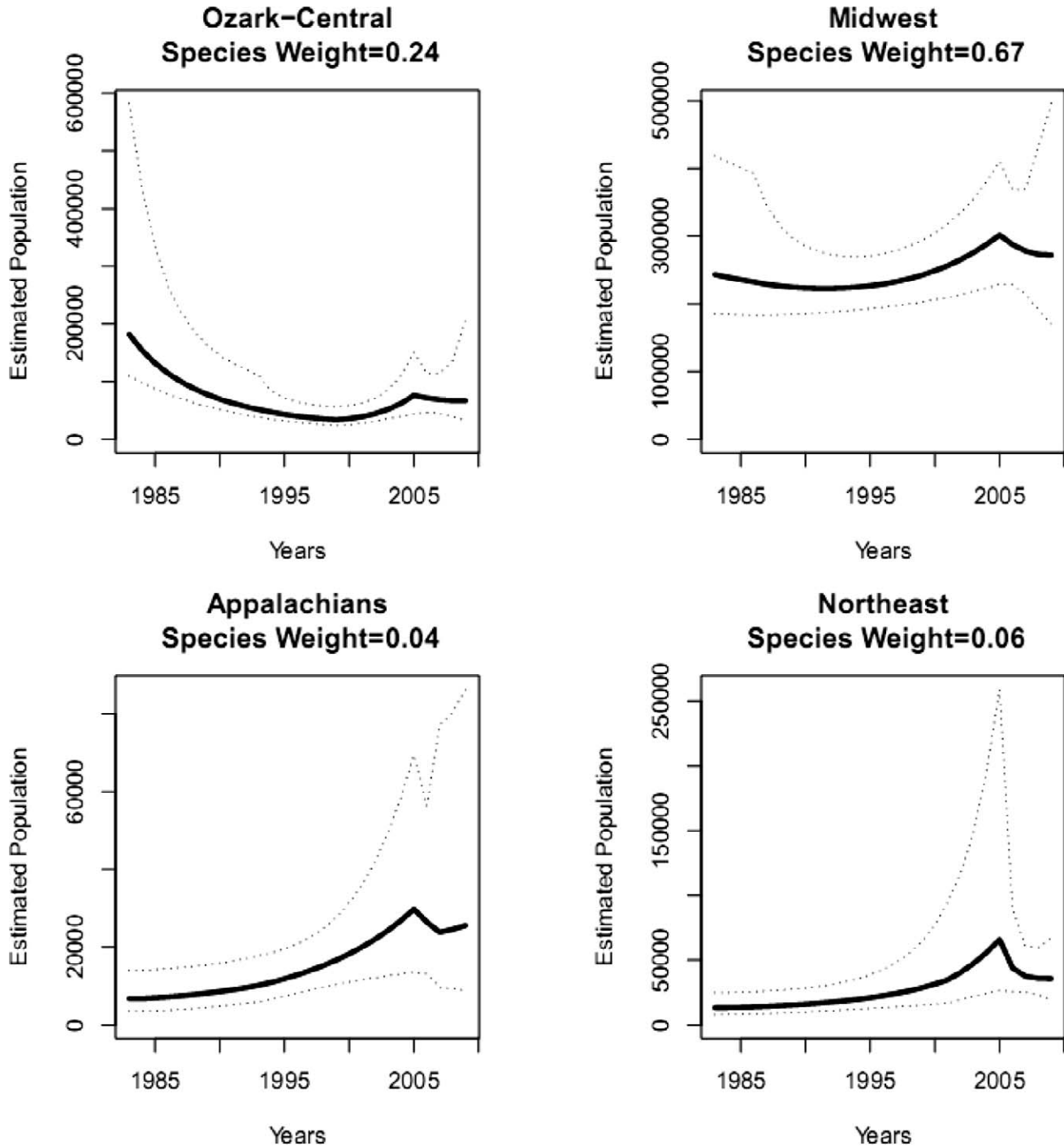
FIG. 4.—Patterns in estimated annual population size of Indiana bats in four recovery units (with 90% CIs). Species weights describe proportional weight of each recovery unit to the total species-level population size estimate.
